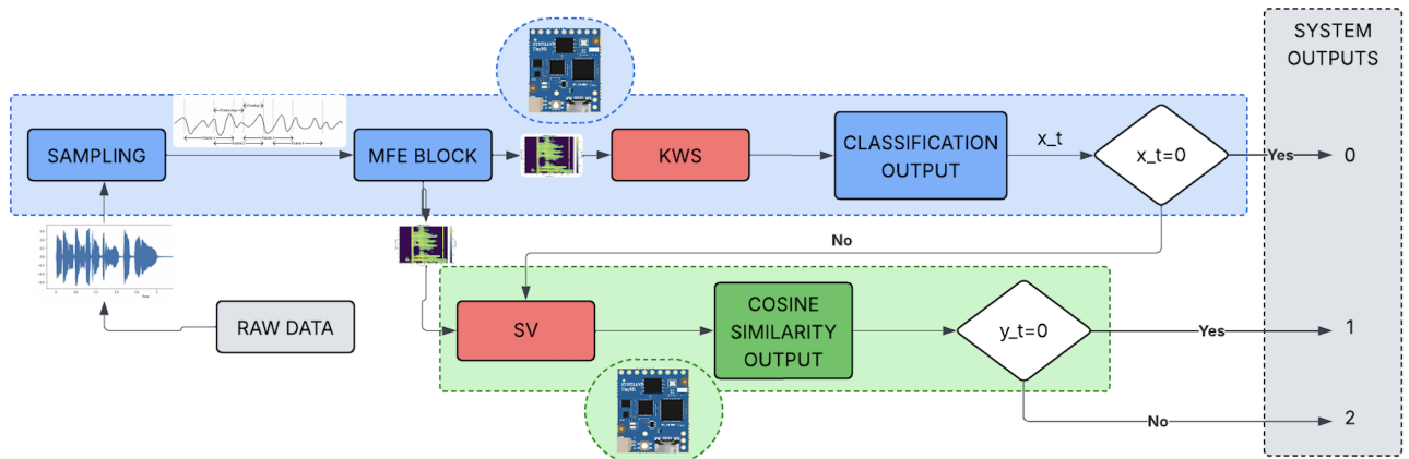
Figure 4.1: Software Pipeline
